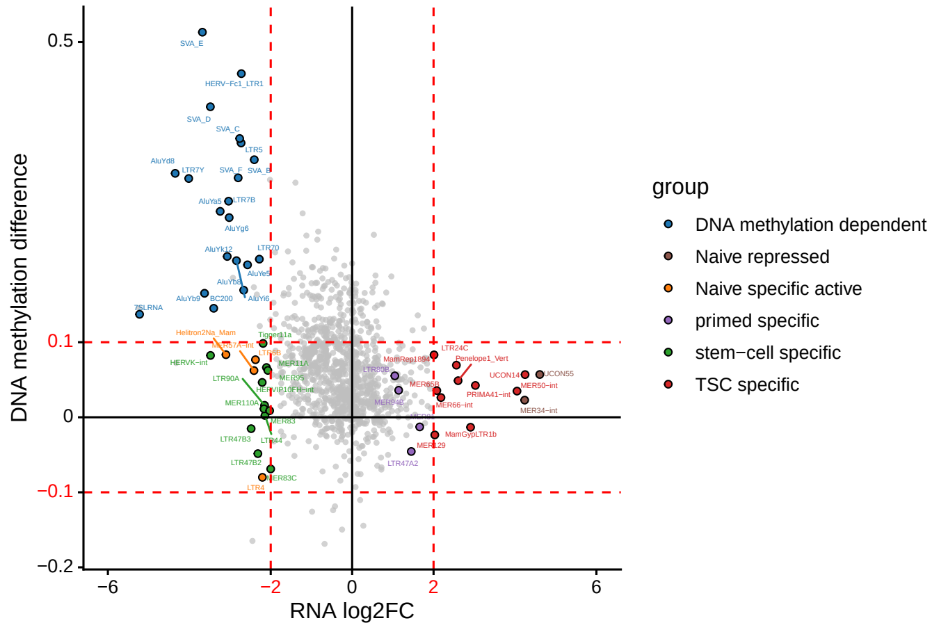
TSC – Naive
