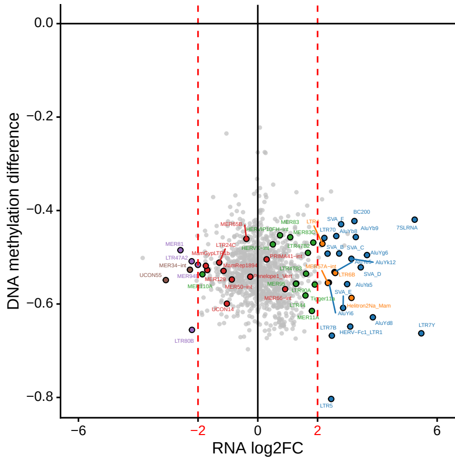
Naive – Primed
