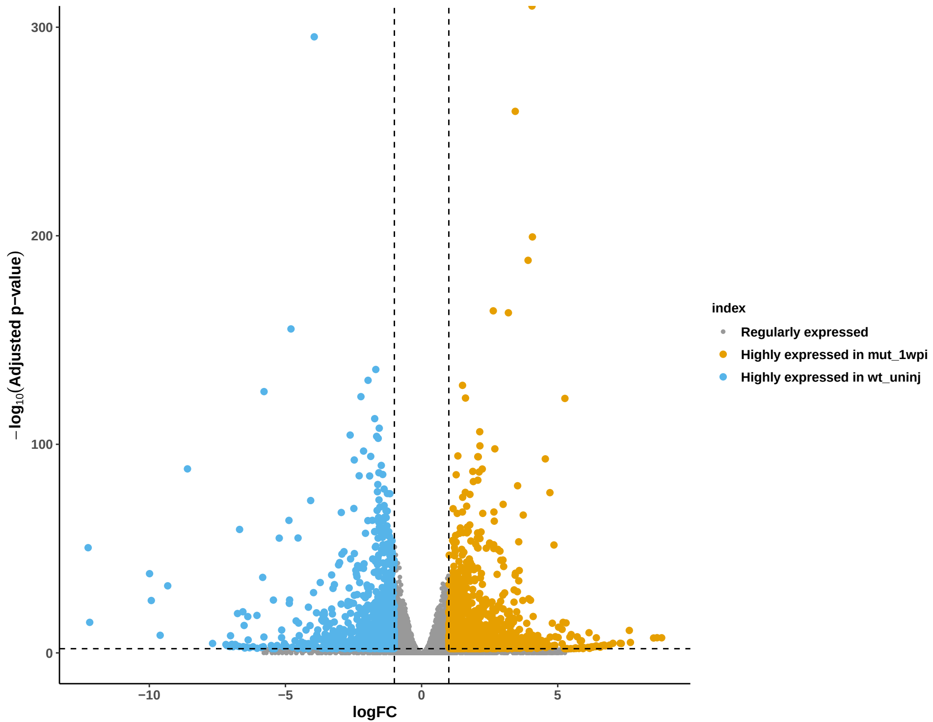
Volcano plot of mut_1wpi vs wt_uninj
