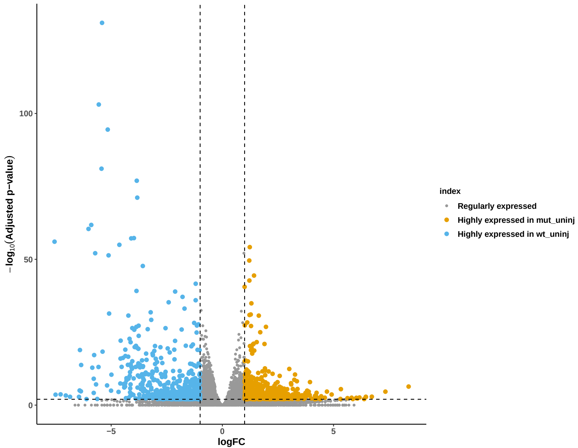
Volcano plot of mut_uninj vs wt_uninj
