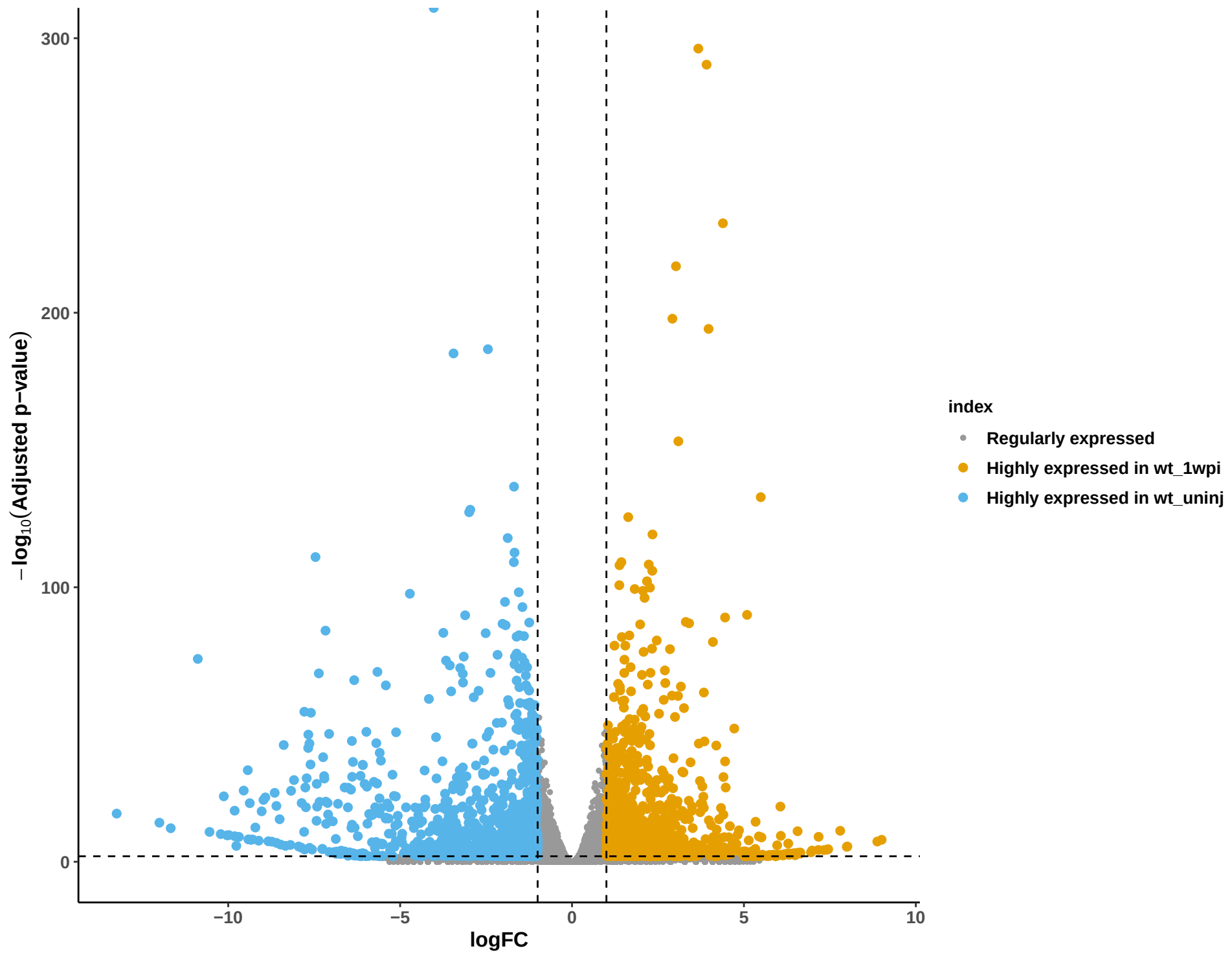
Volcano plot of wt_1wpi vs wt_uninj
