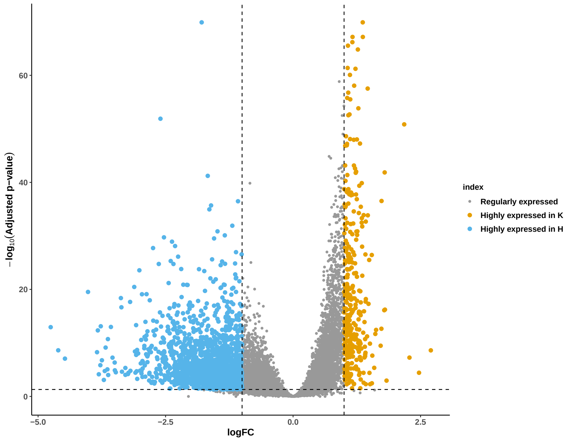
Volcano plot of K vs H
