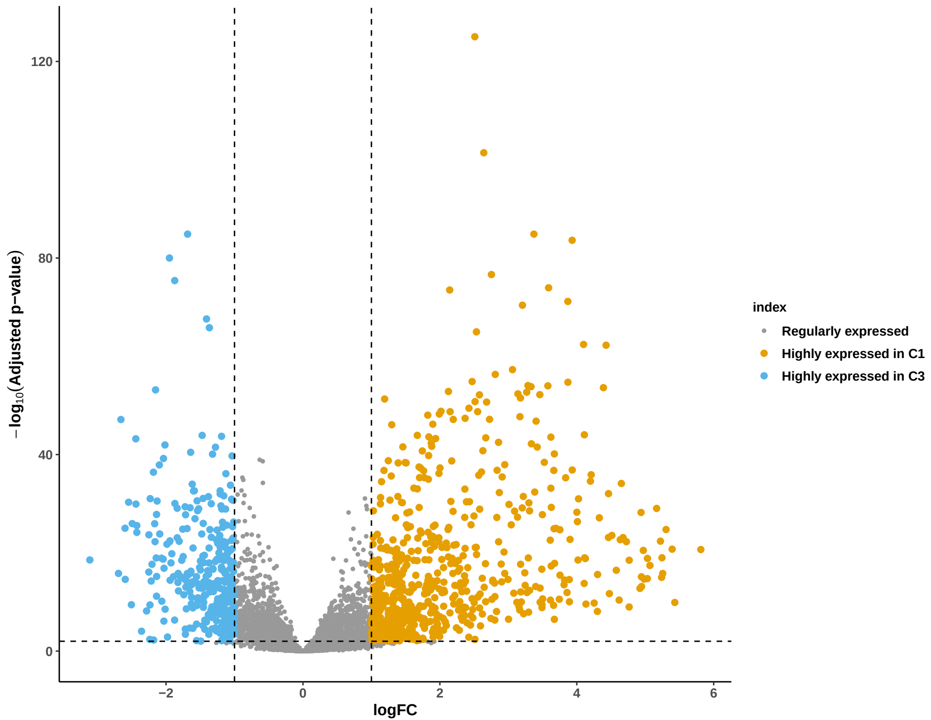
Volcano plot of C1 vs C3
