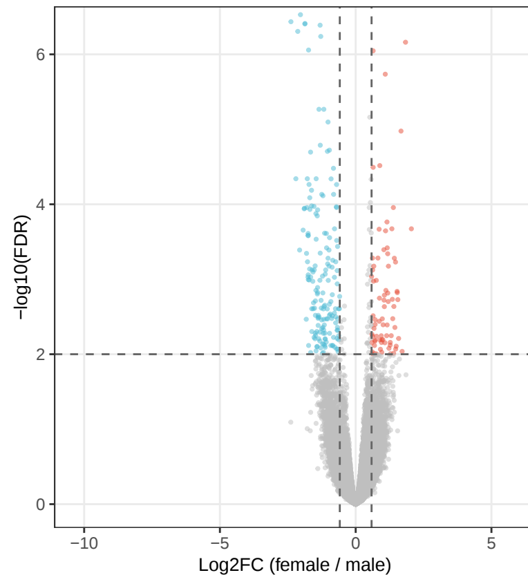
snATAC CM (female vs male, RUVr k=6)
