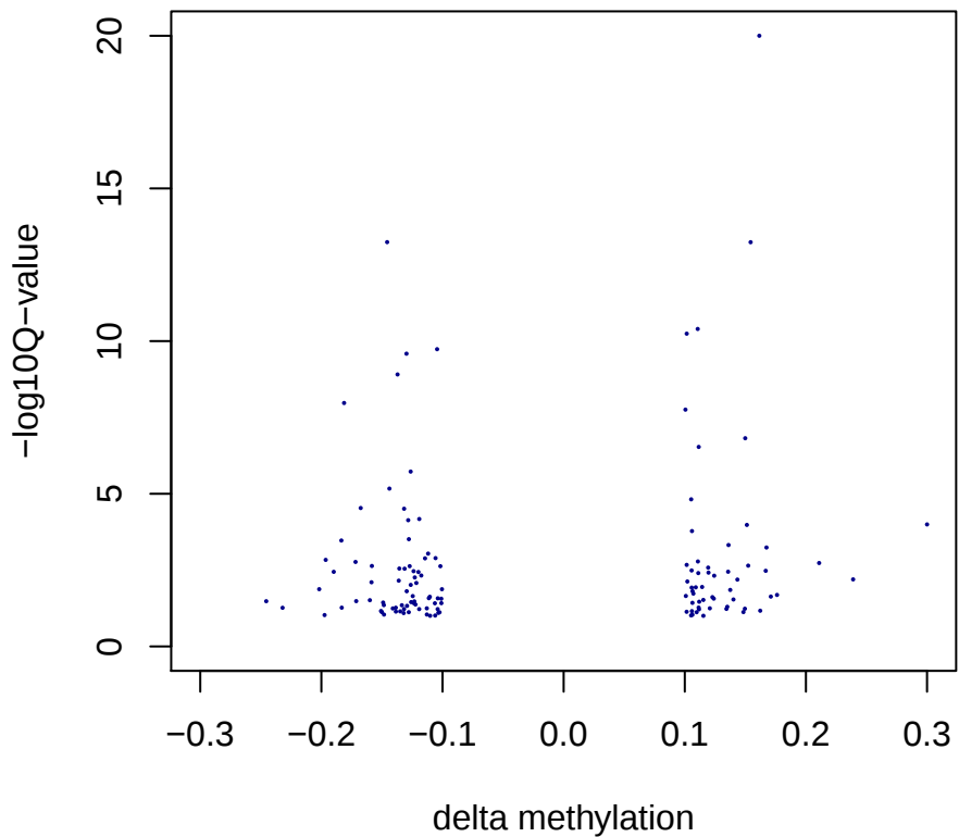
Bins by chisq test of blood_F_As n=130
