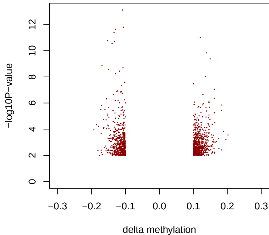
DMRs by metilene of blood_F_As n=1273
