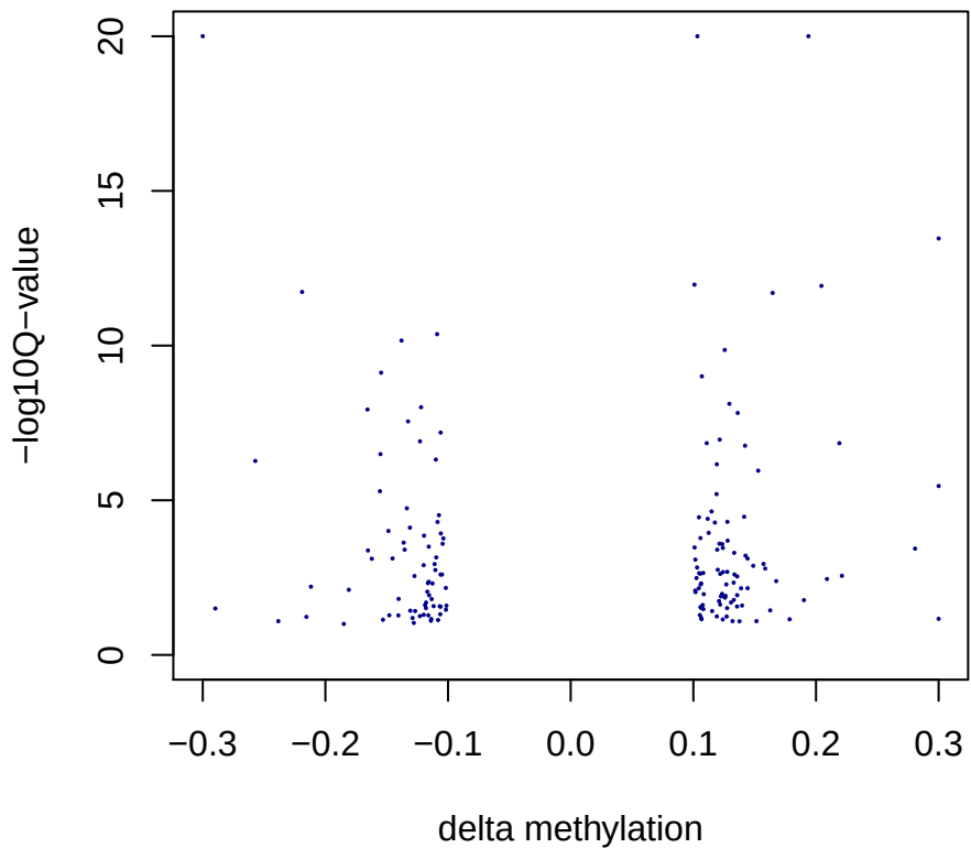
Bins by chisq test of blood_M_Lead n=167
