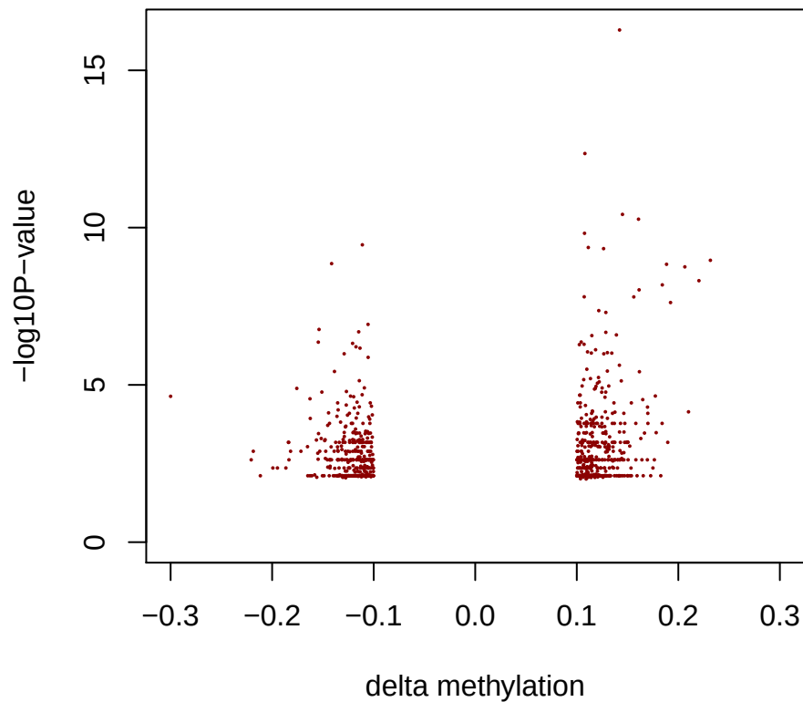
DMRs by metilene of blood_M_Lead n=849
