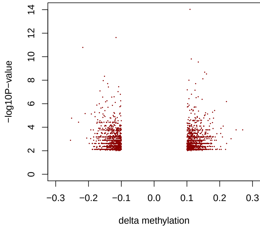
DMRs by metilene of liver_F_Lead n=3211
