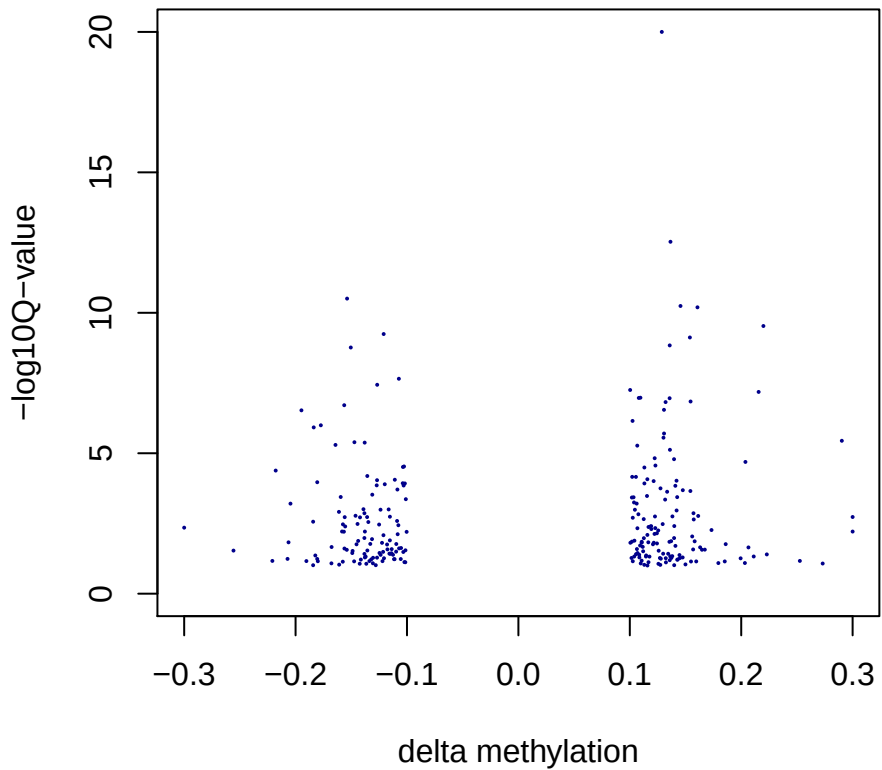
Bins by chisq test of liver_F_Lead n=255
