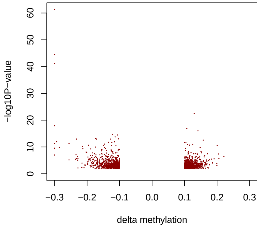
DMRs by metilene of liver_F_TCDD n=2566
