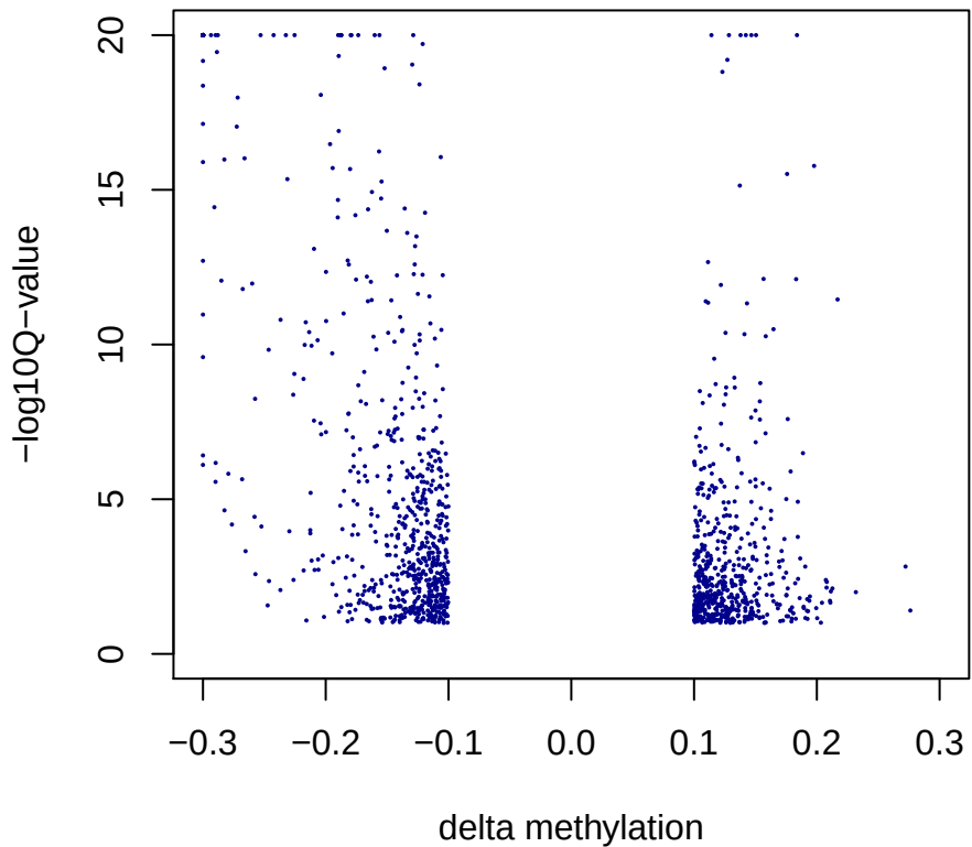
Bins by chisq test of liver_F_TCDD n=1295
