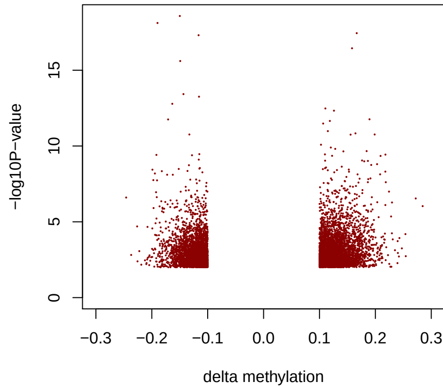
DMRs by metilene of liver_M_As n=7807
