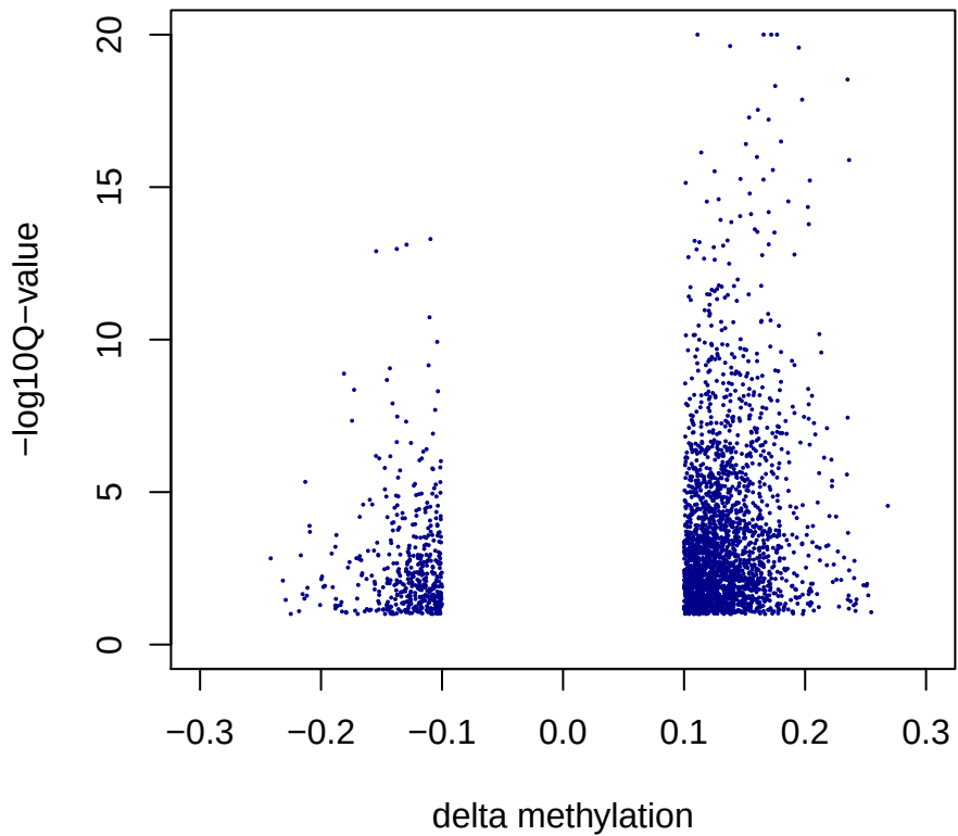
Bins by chisq test of liver_M_As n=2856
