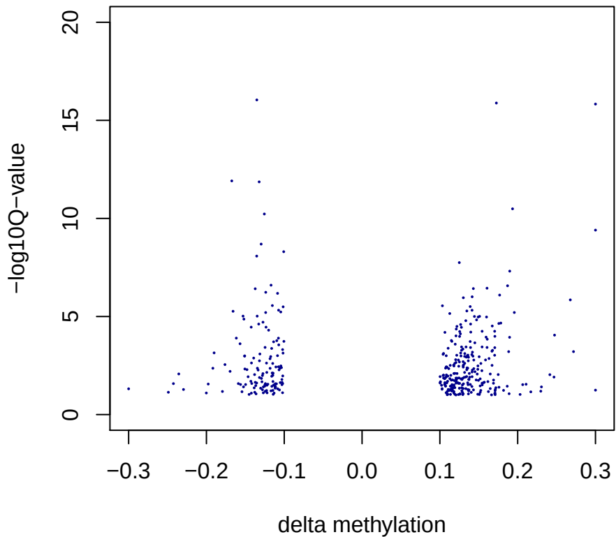
Bins by chisq test of liver_M_DEHP n=391
