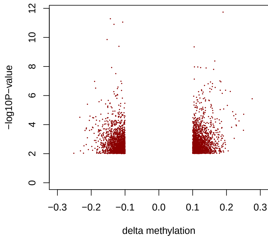
DMRs by metilene of liver_M_DEHP n=3807
