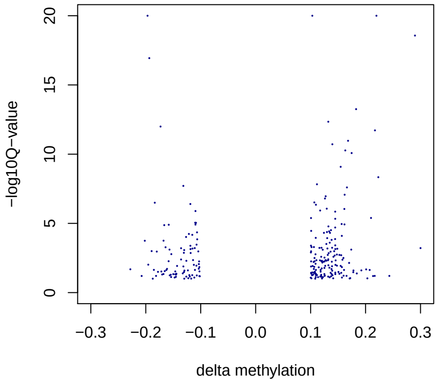
Bins by chisq test of liver_M_Lead n=253
