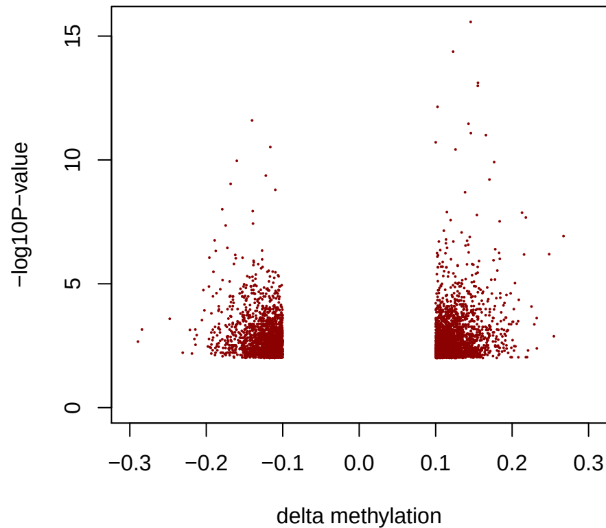
DMRs by metilene of liver_M_Lead n=4385
