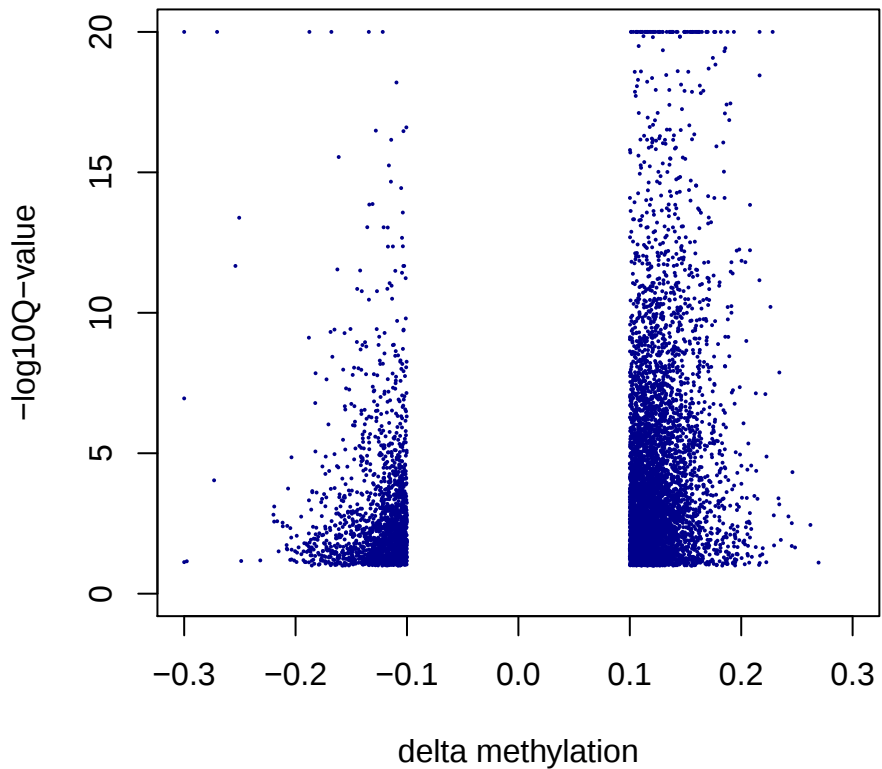
Bins by chisq test of liver_M_TBT n=6986
