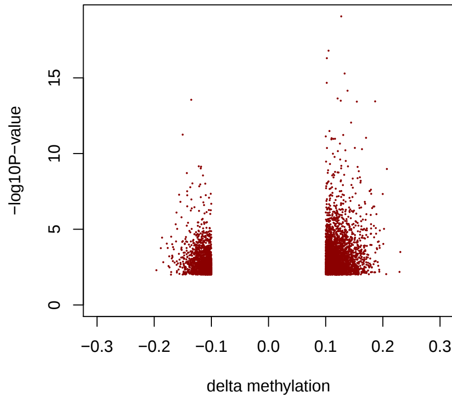
DMRs by metilene of liver_M_TBT n=5099
